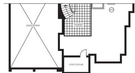
BASEMENT ELEVATION B
