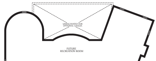
BASEMENT FOR OPTIONAL LOGGIA LAYOUT
