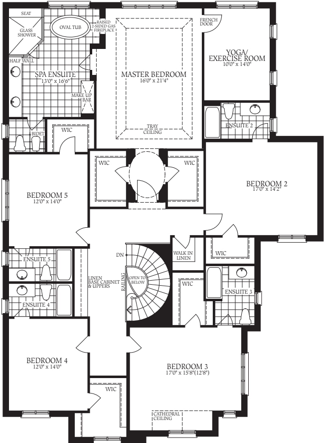
Optional 5 Bedroom Second Floor Elevation A
