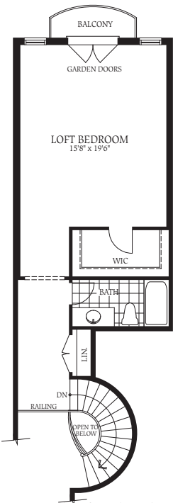
Optional Loft with Bedroom
