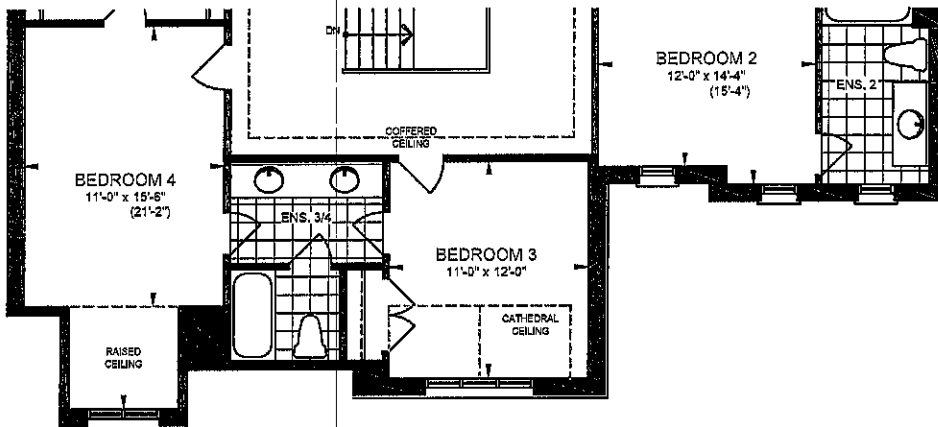
PARTIAL SECOND FLOOR PLAN ELEVATION 'B'
