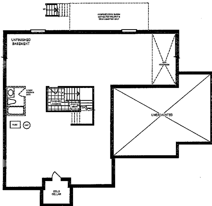
BASEMENT PLAN ELEVATION 'A'
