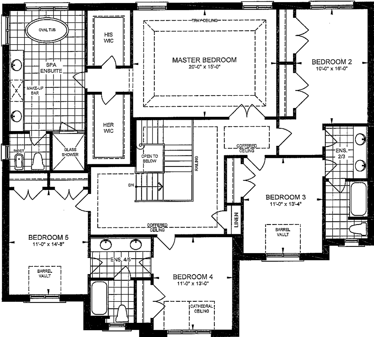
OPTIONAL 5 BEDROOM SECOND FLOOR PLAN ELEVATION 'A'
