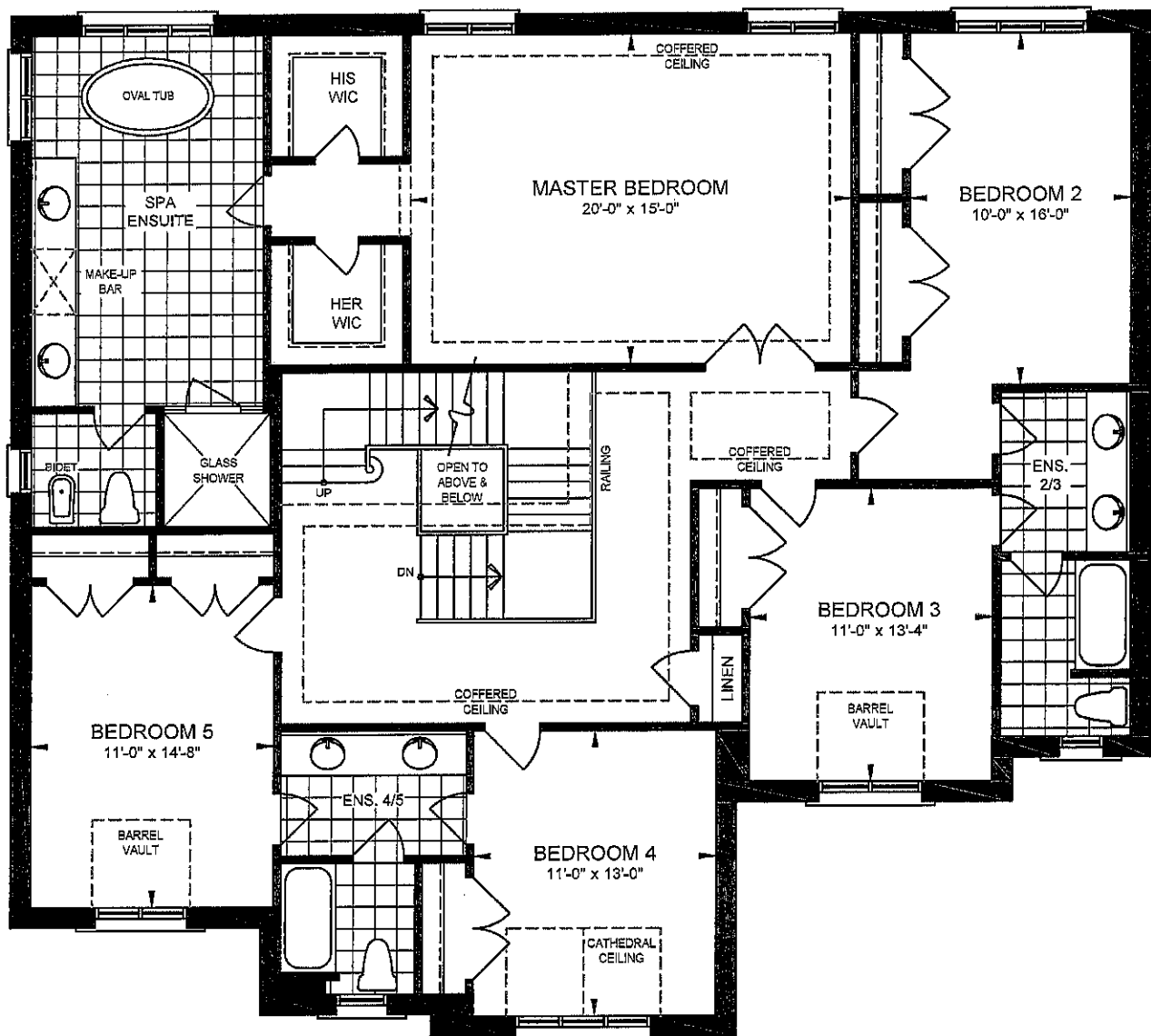
OPTIONAL 5 BEDROOM SECOND FLOOR PLAN W/ OPTIONAL LOFT ELEVATION 'A'
