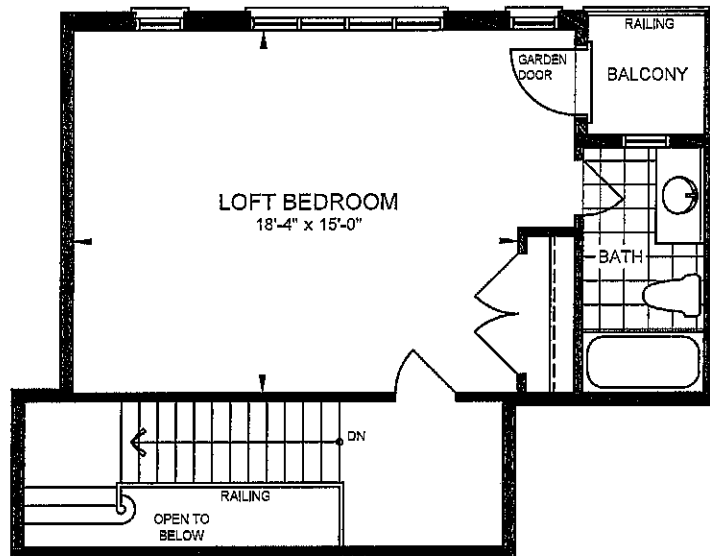
OPTIONAL LOFT PLAN W/ BEDROOM ELEVATION 'A' & 'B'
